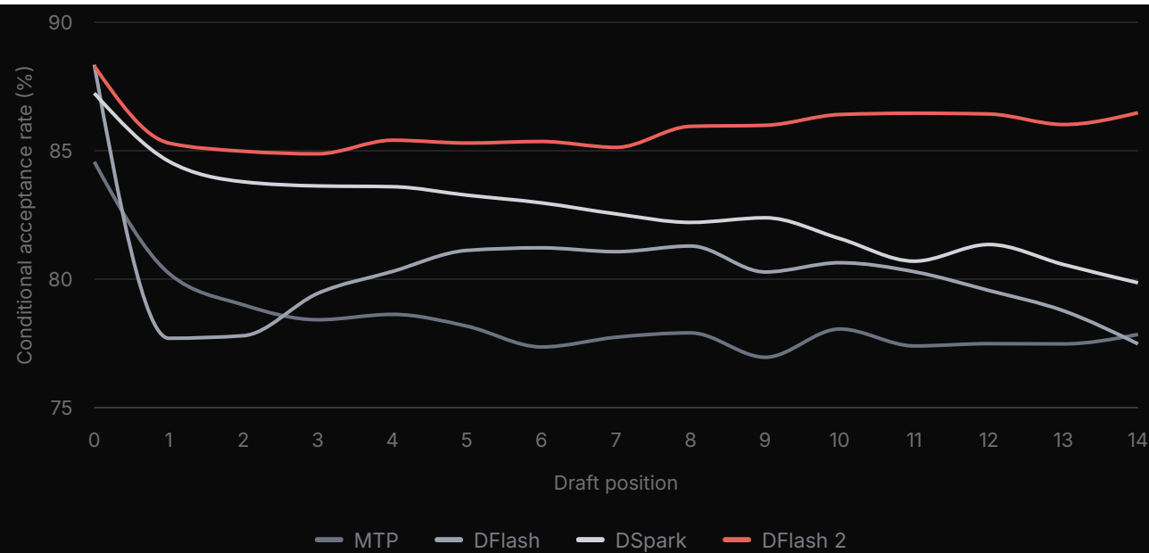
Figure 5. Qwen3.5-4B conditional acceptance rate on MATH-500, same sampling as above.
