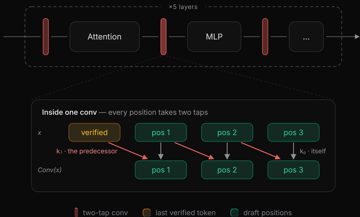
Figure 4. The two-tap dynamic convolution. One sits before and after each attention and MLP sublayer of every drafter layer. Inside it, each position mixes its own representation with its predecessor's, and the first position reads the last verified token.
