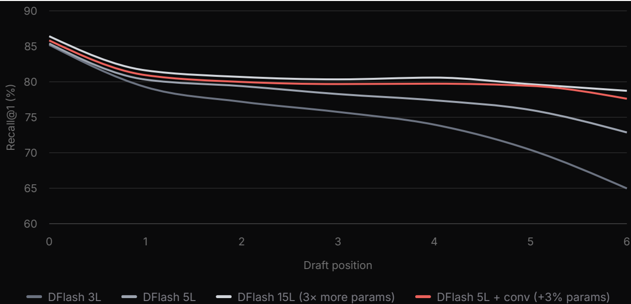
Figure 2. Qwen3-4B Recall@1 on GSM8K at T=0, conditioned on every earlier position being right. All drafters are trained under the same setup; the convolutional model is evaluated without the selector. Its convolutions add 3% parameters and 0.7% cycle latency; the ten extra layers of 15L add 15.2%.
