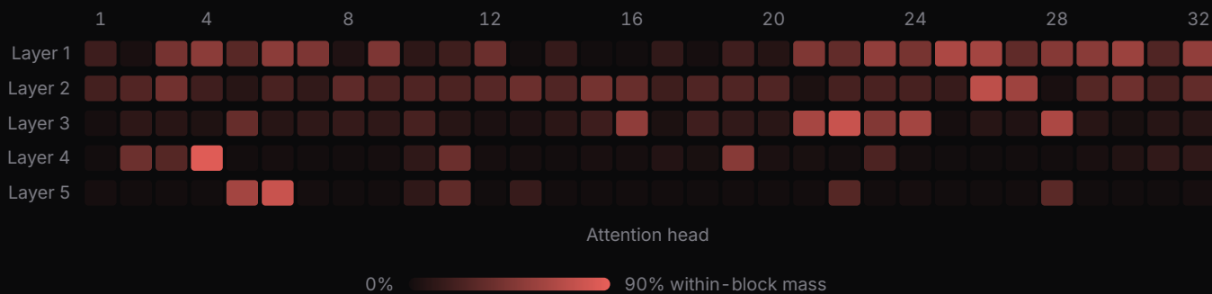
Figure 3. Within-block attention by head in five-layer Qwen3-4B DFlash. Brighter cells mark heads that spend more attention on the draft block; in later layers the within-block mass shrinks and concentrates in a few heads.
