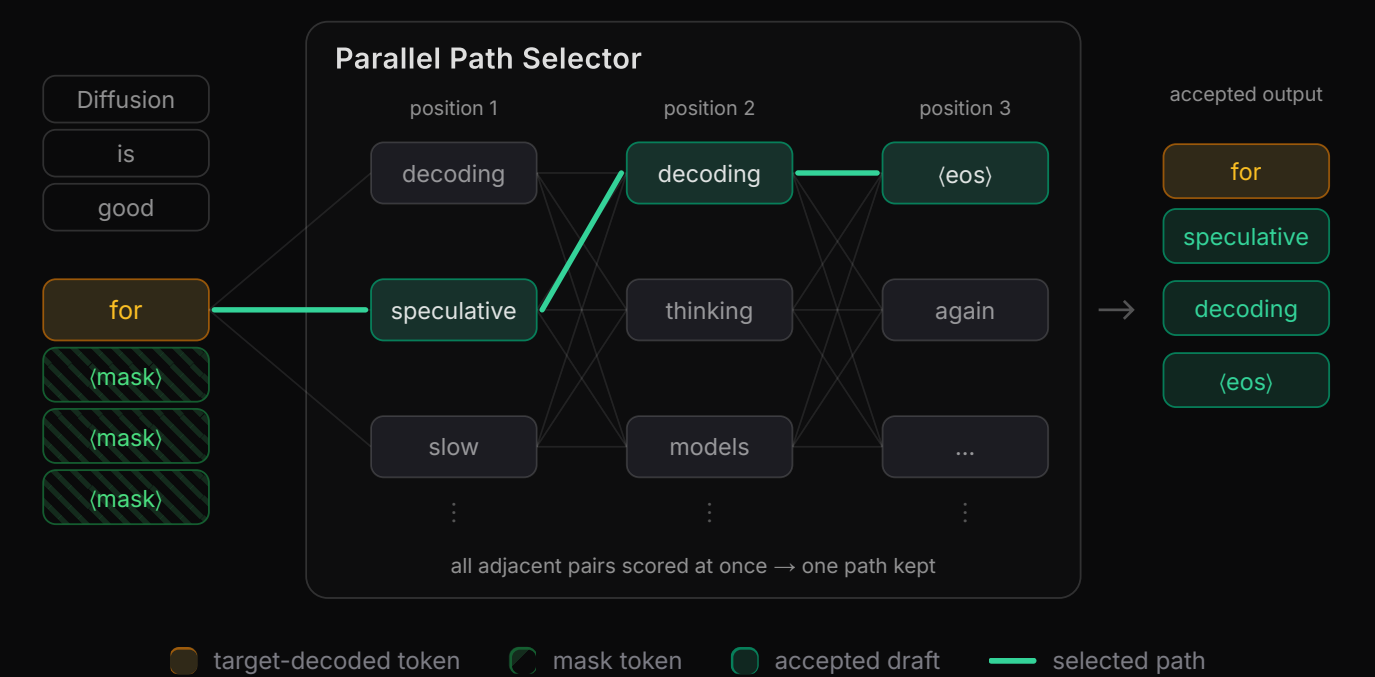
Figure 1. The selector in one cycle. With DFlash alone, each position keeps its top pick; here two neighbors both pick the same word, and the stutter dies at verification. DFlash 2 keeps each position's top candidates, and the selector traces one coherent path through them; here, the whole block survives.
